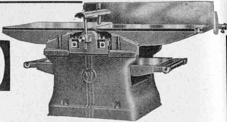
12" x 4" Combined Planing and Thickening machine type PTJ.
