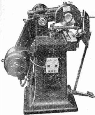
SAWING MACHINES
